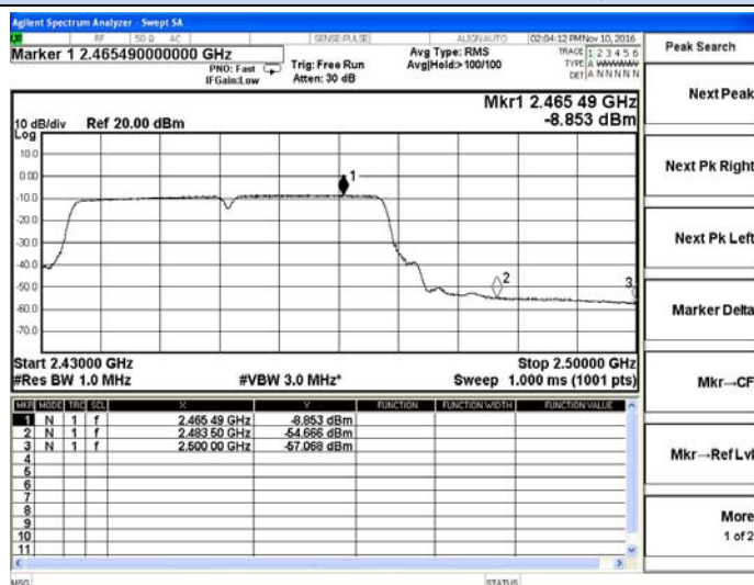
802.11n(HT40)-High channel(Average)
