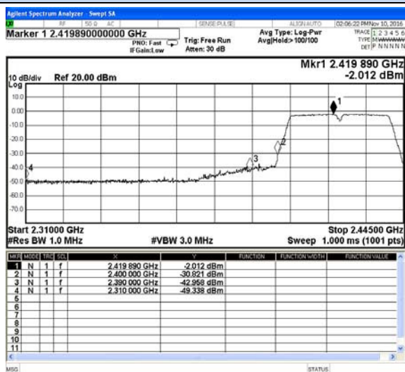
802.11n(HT40)-Low channel(Peak)
