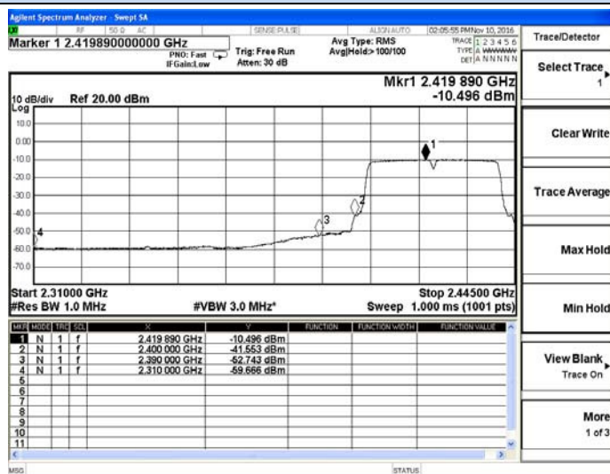
802.11n(HT40)-Low channel(Average)
