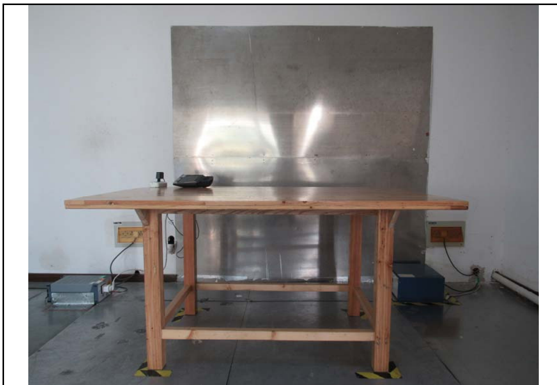
Conducted Emissions Test Setup Front View
