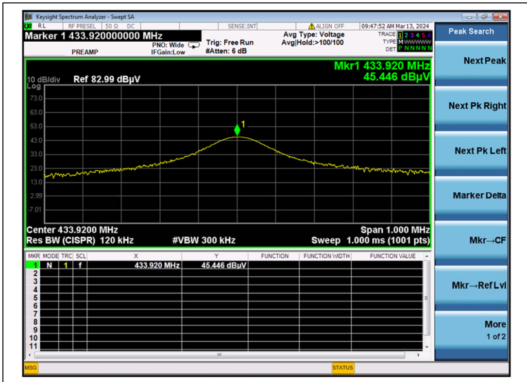
(Antenna Vertical)
