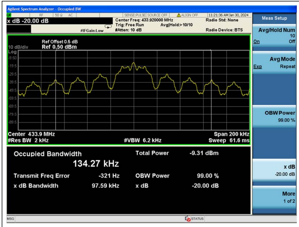
(Bandwidth)
