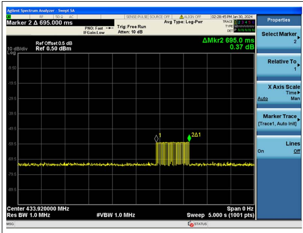
(The max transmission time)
