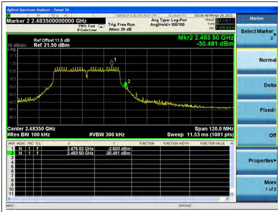
(Band Edge, Channel 11, 802.11n (HT40))
