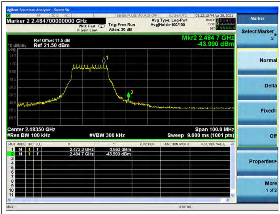
(Band Edge, Channel 12, 802.11g)
