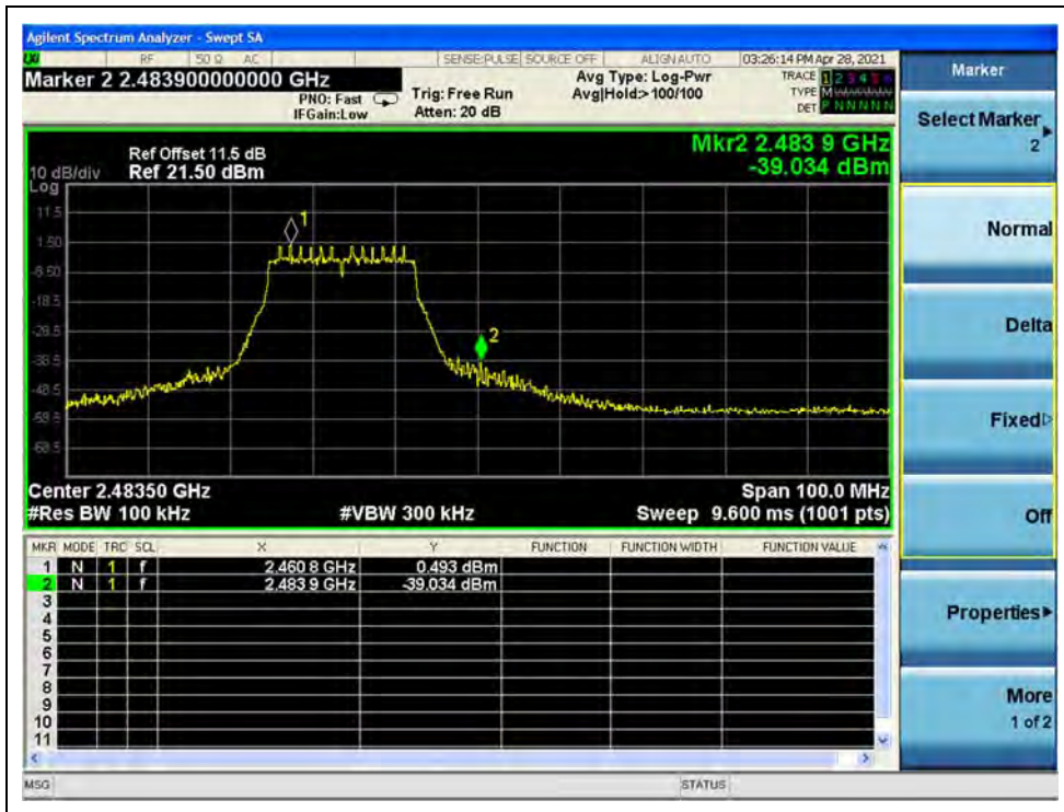
(Band Edge, Channel 12, 802.11n (HT20))
