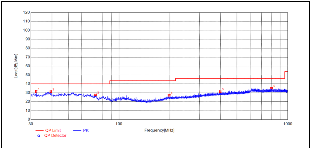
(30MHz – 1GHz, Test Antenna Vertical)
