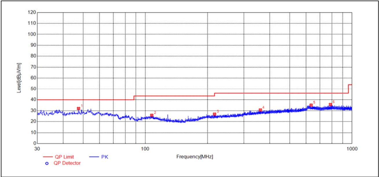
(30MHz – 1GHz, Test Antenna Vertical)
