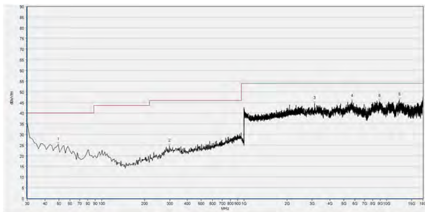
(30MHz to 18GHz, Antenna Horizontal, 8-DPSK, channel 39)
