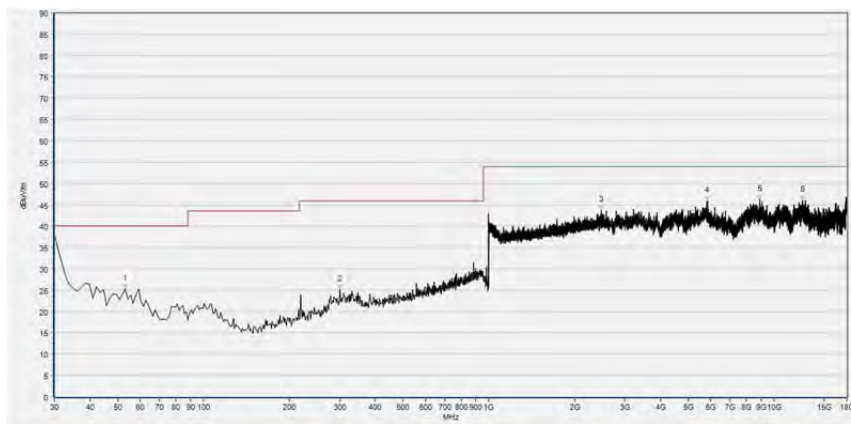
(30MHz to 18GHz, Antenna Horizontal, \pi/4 -DQPSK, channel 78)
