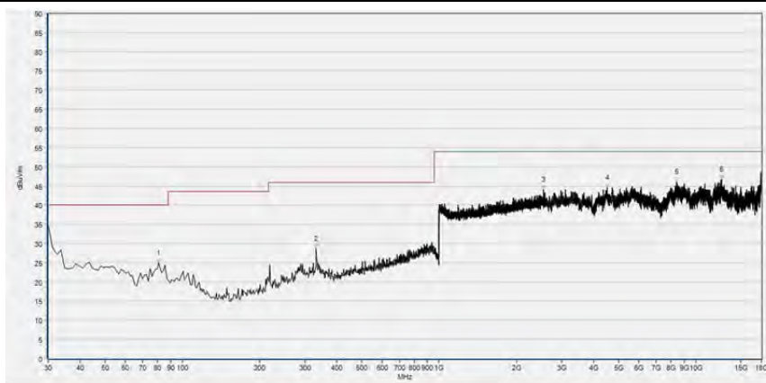
(30MHz to 18GHz, Antenna Horizontal, GFSK, channel 78)
