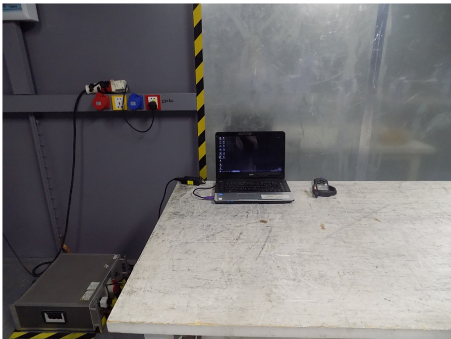
Photos of POWER LINE CONDUCTED EMISSION
