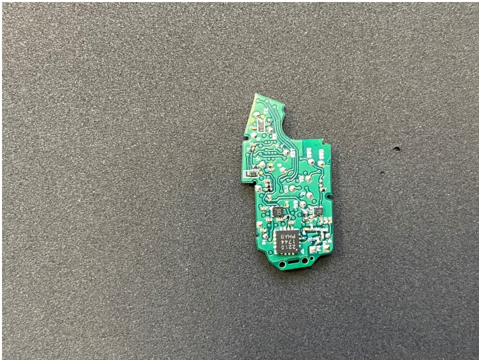
Right Hearing Aid PCB Bottom View
