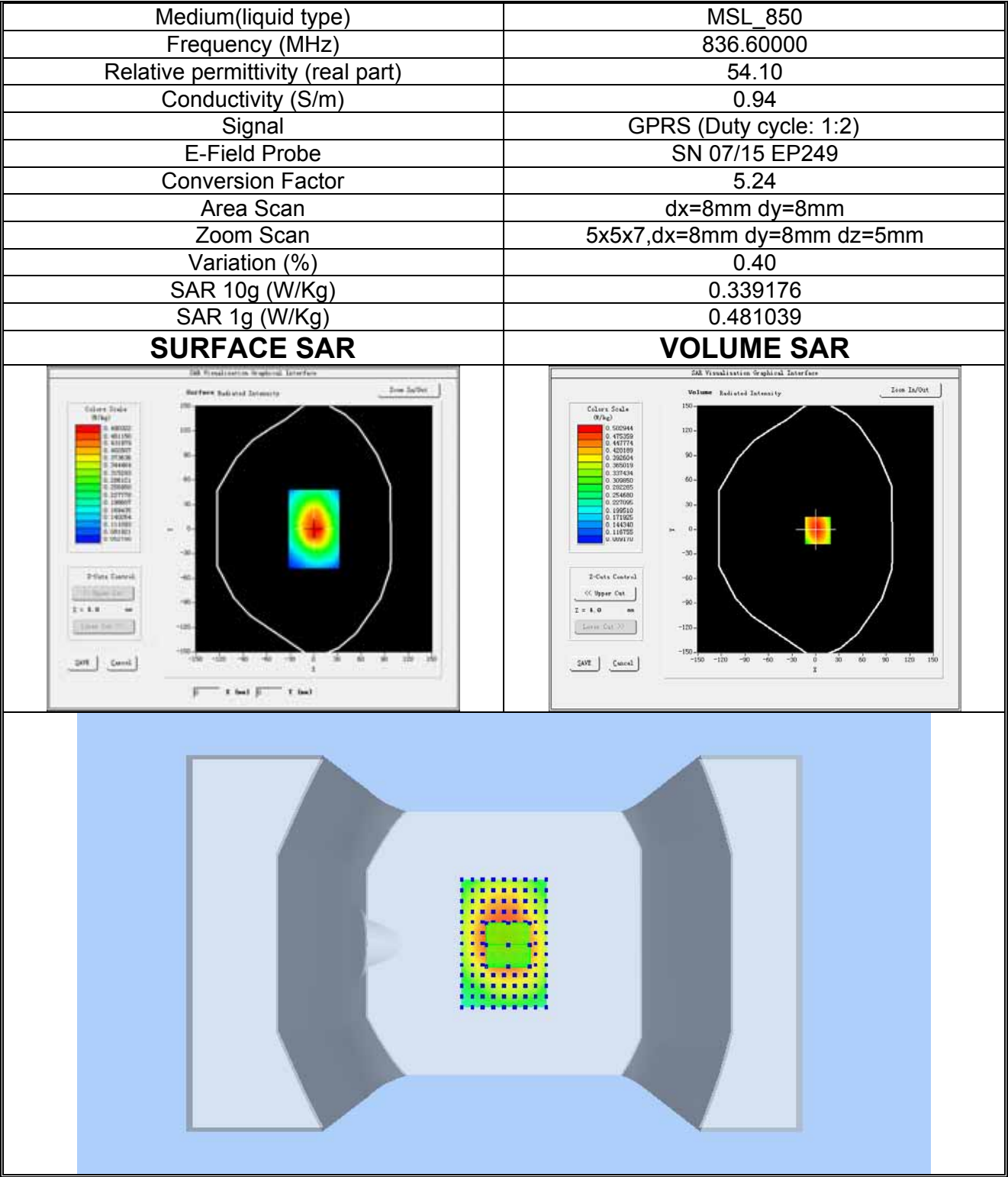
Plot 7: GPRS850MHz, Mid channel (Body-worn, Right edge) Product Description: Mobile Phone Test Date: 2018-05-30
