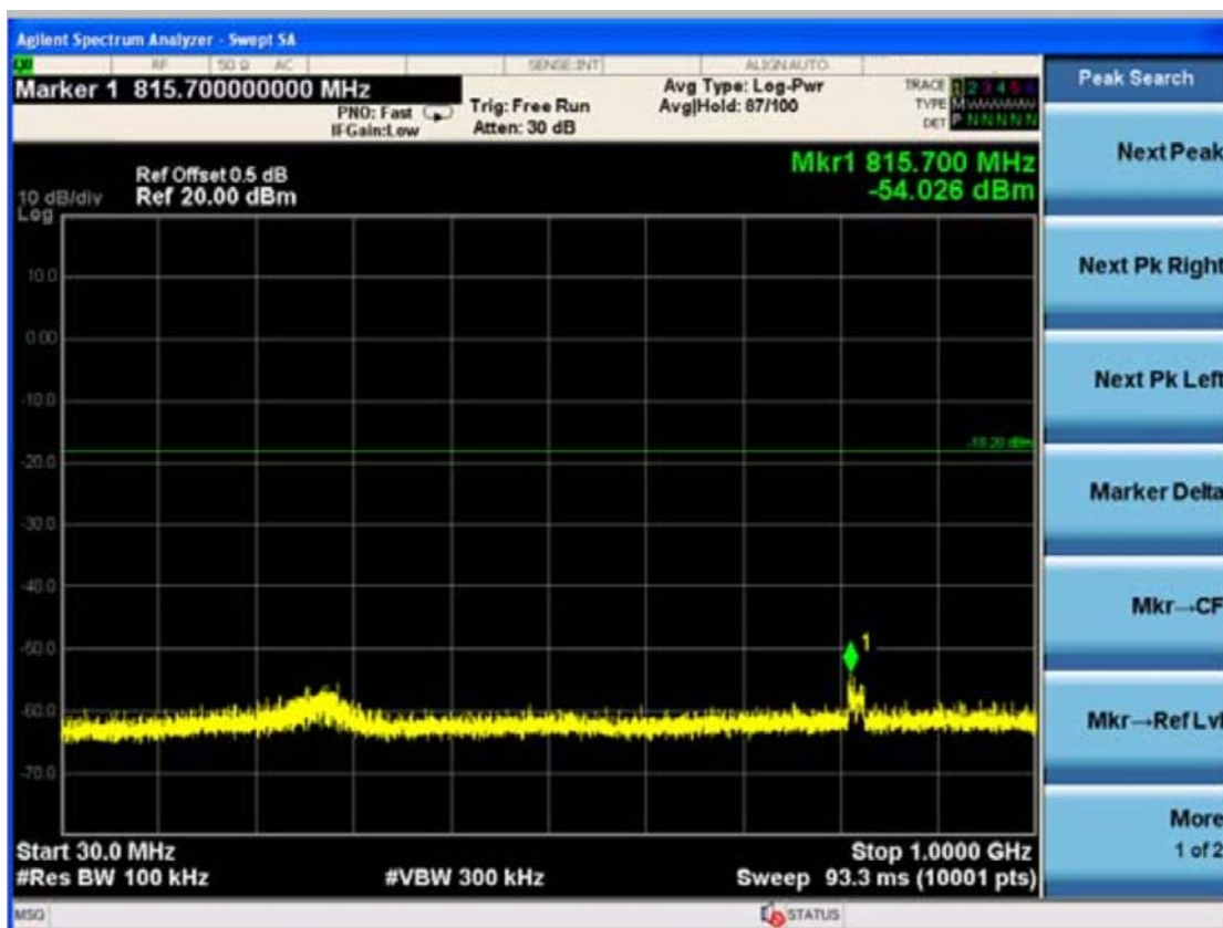
TX 802.11g Mode CH11
