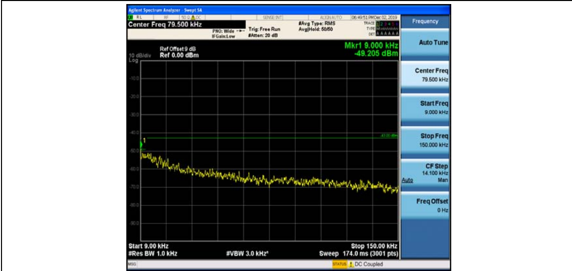
Band25_1.4MHz_QPSK_26365_1RB#0
