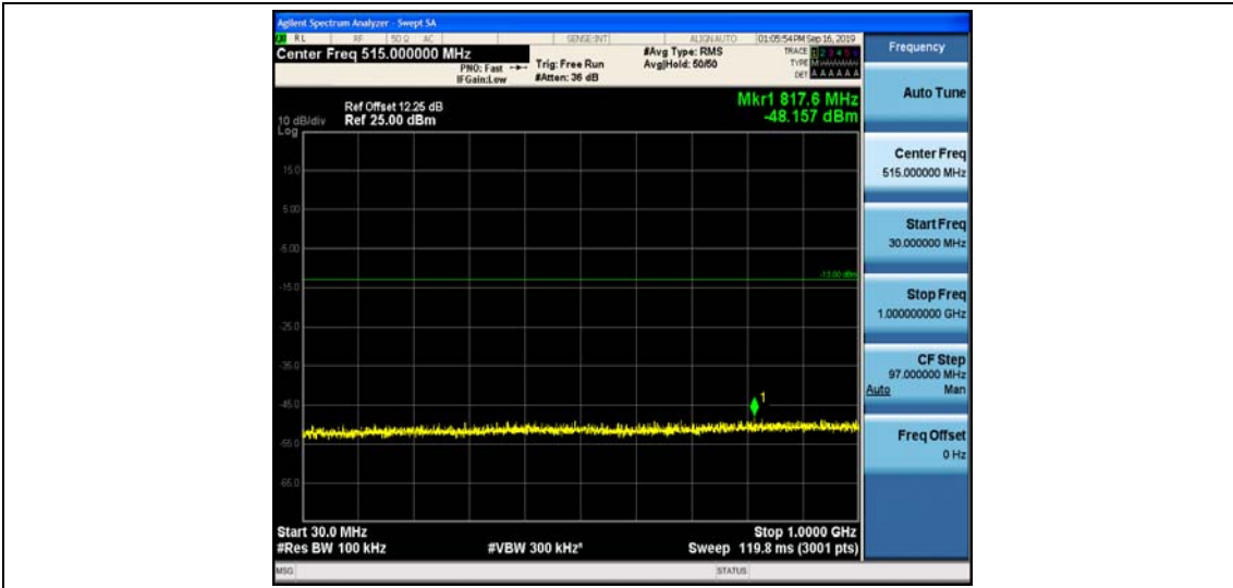
Band66_1.4MHz_QPSK_132322_1RB#0
