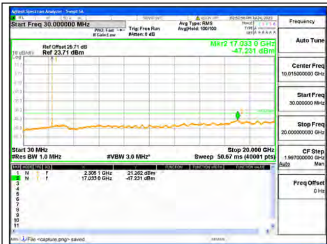
B30-30M-20G / 10MHz / Low CH / QPSK
