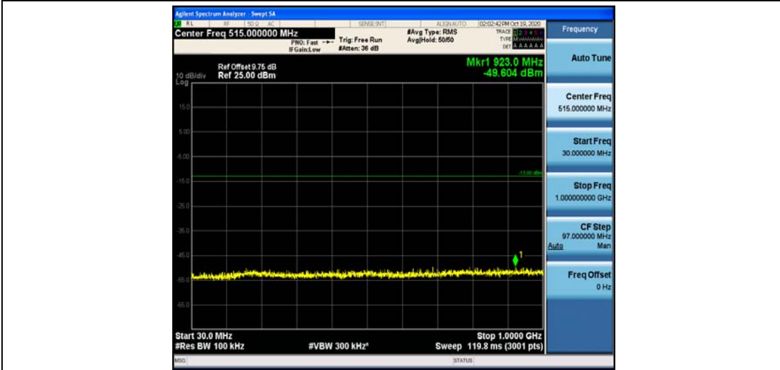
Band66_3MHz_QPSK_132657_1RB#0
