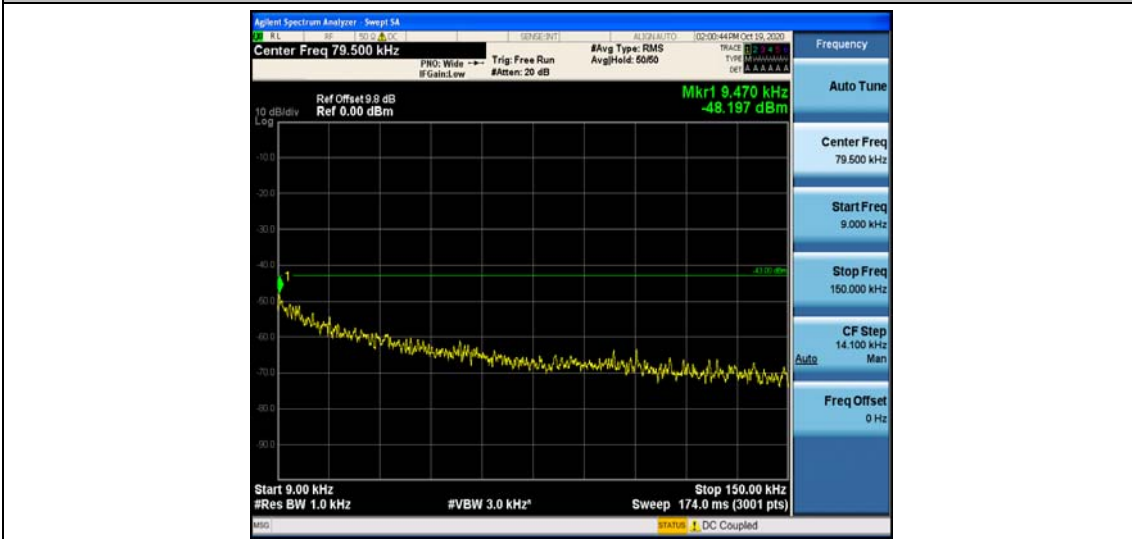
Band66_3MHz_16QAM_132322_1RB#0
