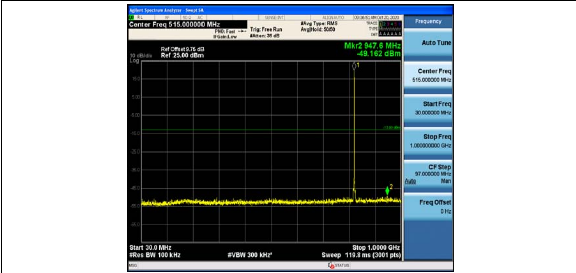
Band26_1.4MHz_16QAM_26797_1RB#0
