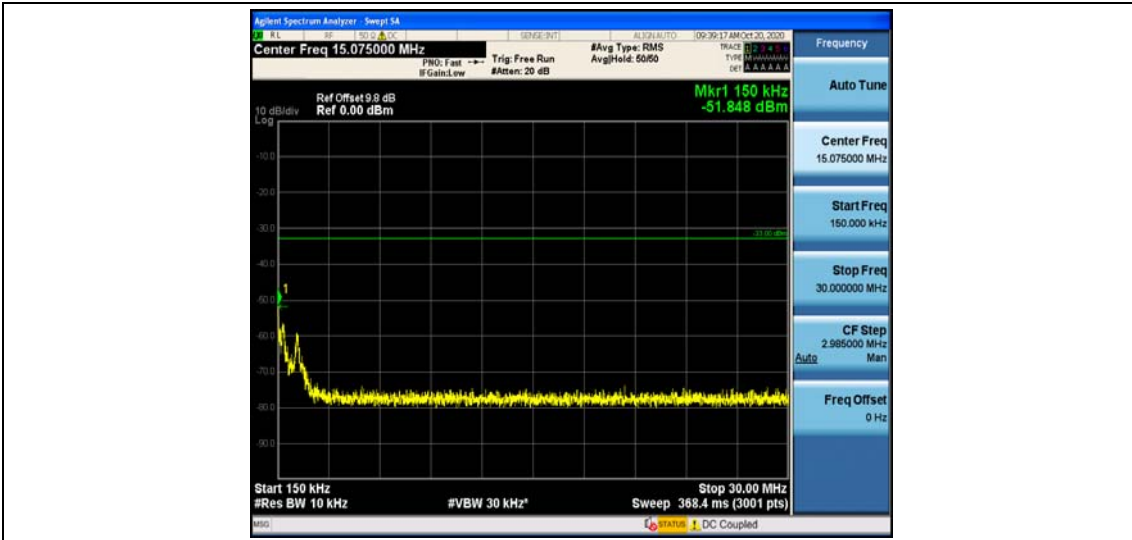
Band26_1.4MHz_16QAM_26915_1RB#0
