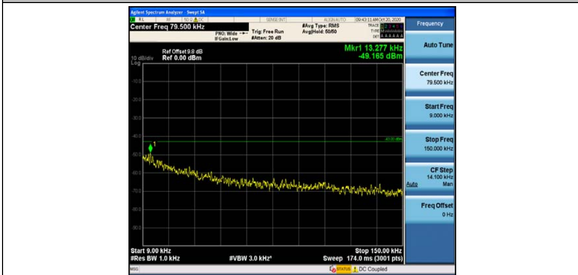
Band26_3MHz_QPSK_26805_1RB#0
