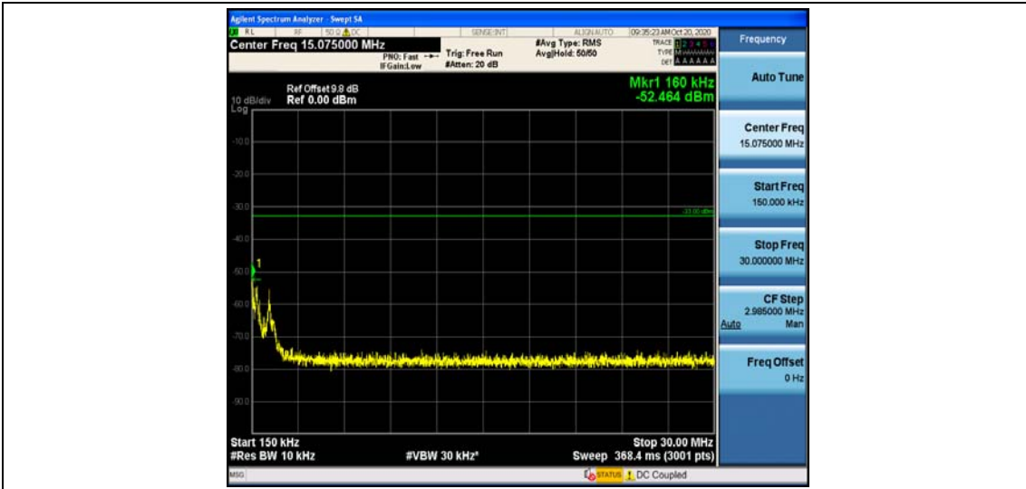
Band26_1.4MHz_QPSK_26797_1RB#0
