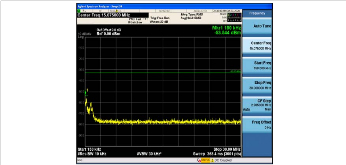
Band26_1.4MHz_16QAM_26797_1RB#0
