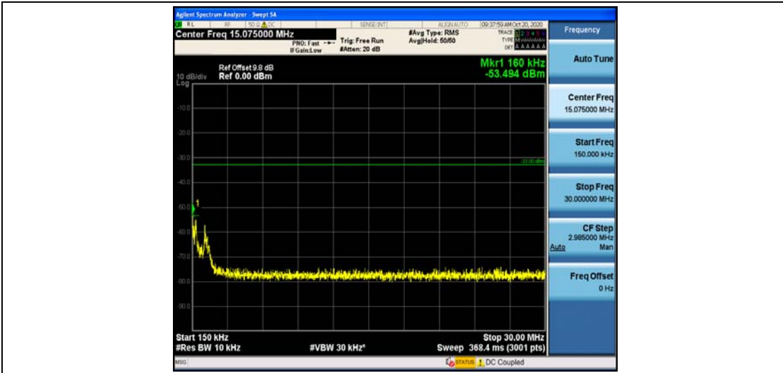
Band26_1.4MHz_QPSK_26915_1RB#0
