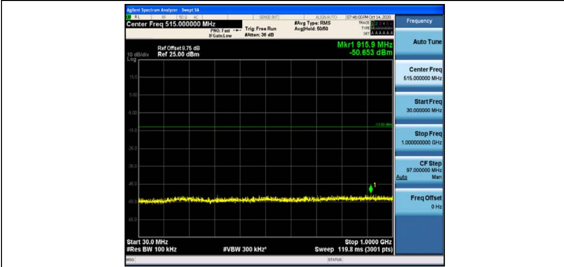
Band25_3MHz_16QAM_26365_1RB#0
