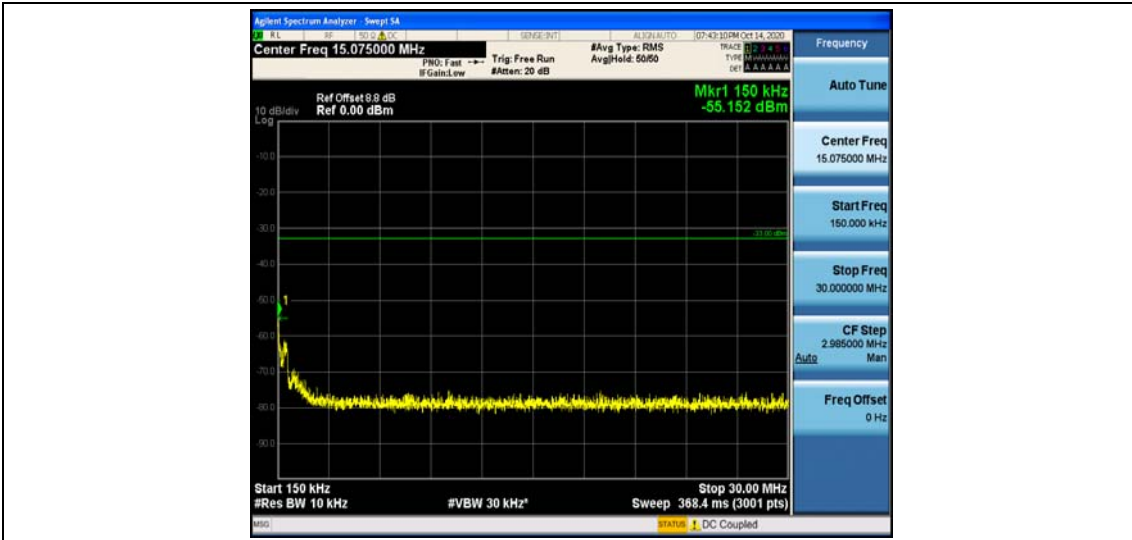
Band25_3MHz_16QAM_26055_1RB#0
