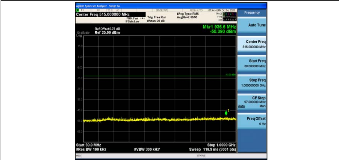
Band25_3MHz_QPSK_26365_1RB#0
