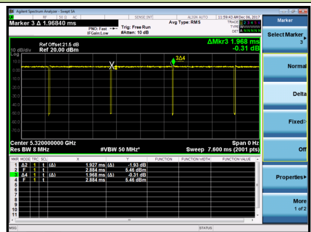
802.11ac-VHT20 - T = 1.927 ms
