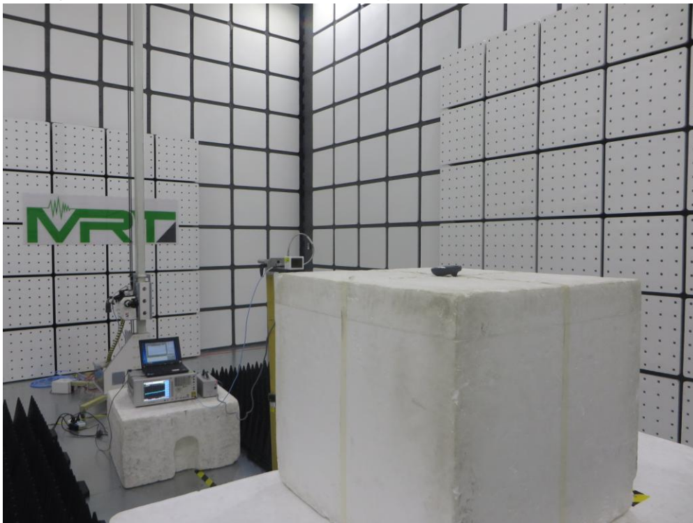
Description: Radiated Emissions Test Setup for Above 18GHz
