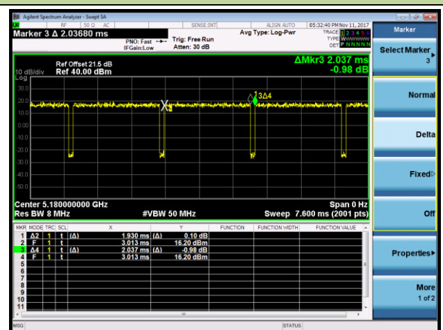
802.11ac-VHT20 - T = 1.930 ms
