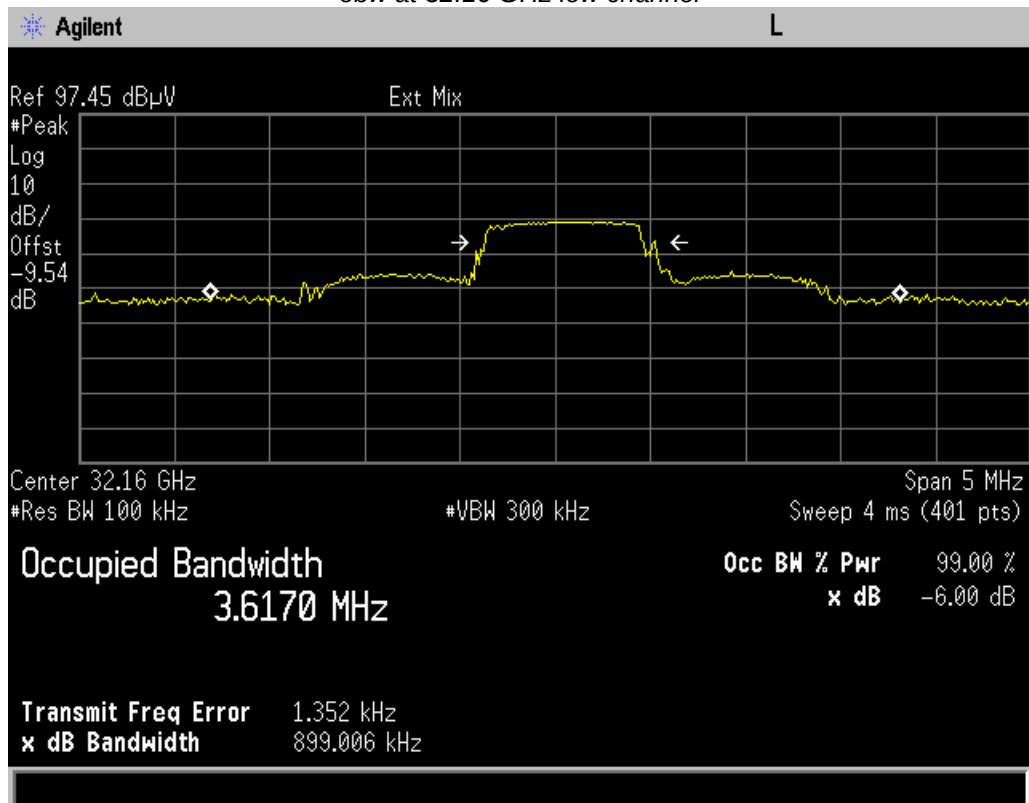
obw at 32.16 GHz low channel
