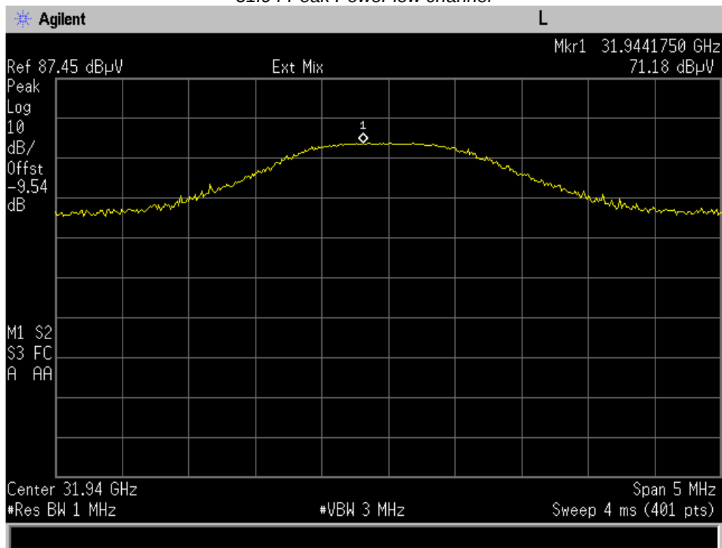
31.94 Peak Power low channel
