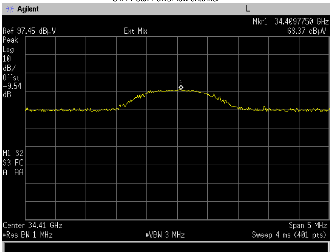
34.4 Peak Power low channel
