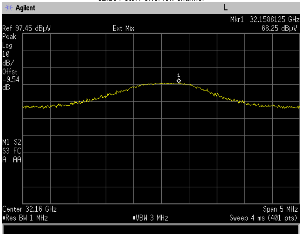
32.16 Peak Power low channel
