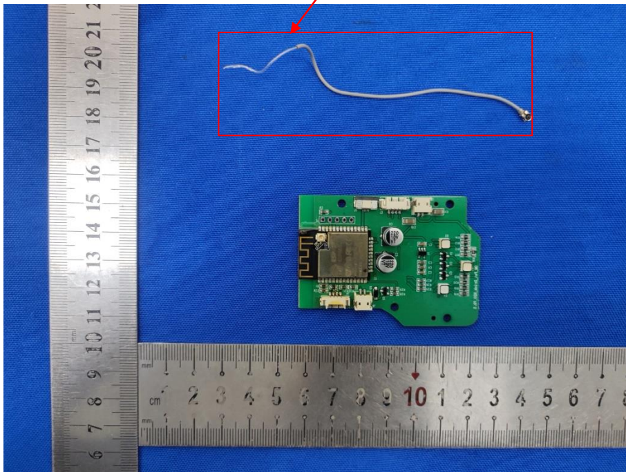
2.4G/BLE Antenna
