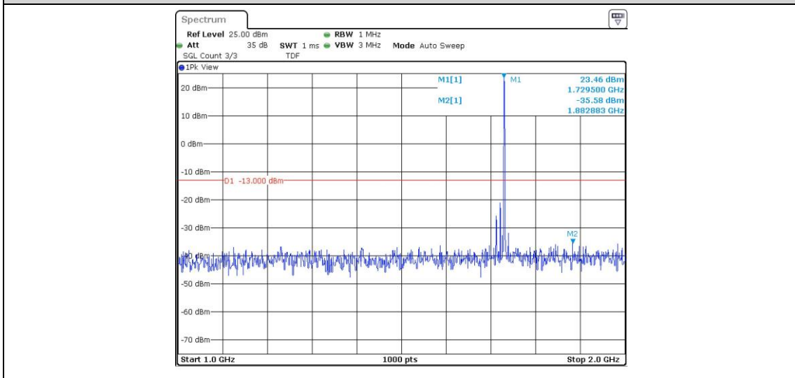
Band4-20MHz-16QAM-20050-1RB#99-Range3:2000~20000MHz
