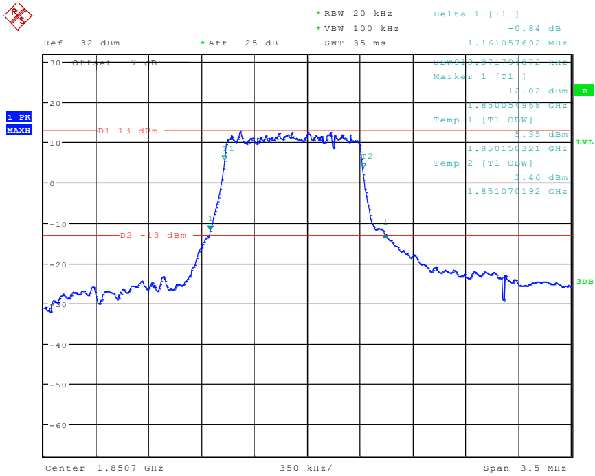
2 Band 2_1.4 MHz_Low_16QAM_RB5#0
