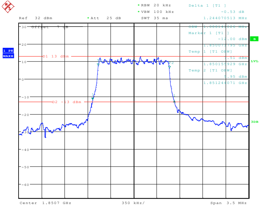
1 Band 2_1.4 MHz_Low_QPSK_RB6#0
