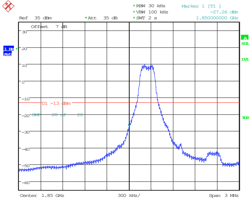
1 Band 2_1.4 MHz_Low_QPSK_RB1#0
