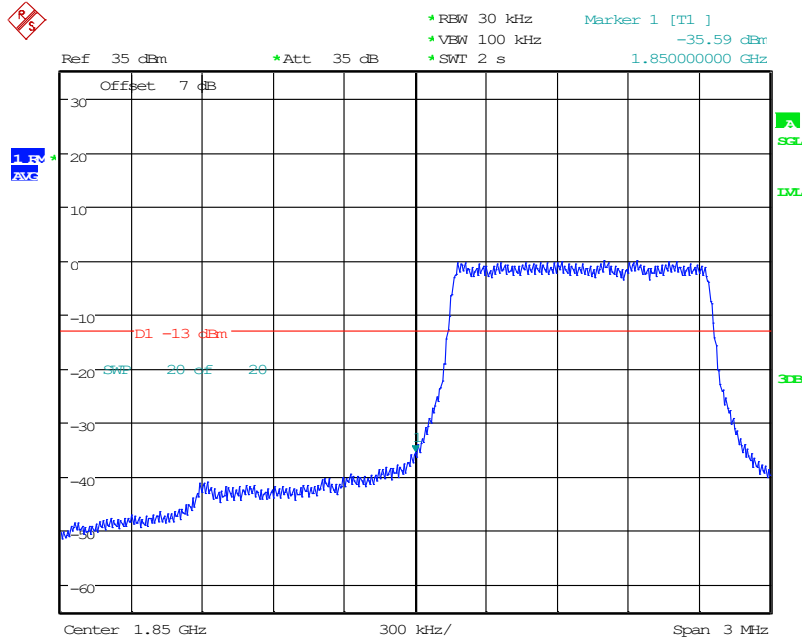
2 Band 2_1.4 MHz_Low_QPSK_RB6#0
