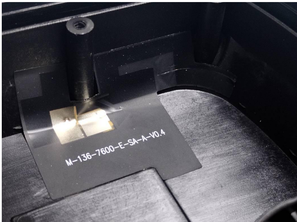
3G/4G Antenna
