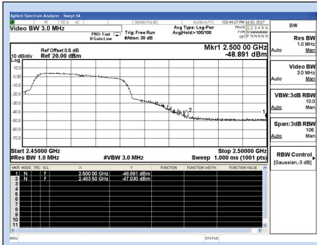
Channel 1 / 2462 MHz – Peak
