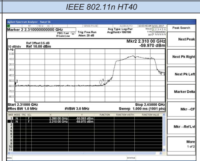
Channel 11 / 2422 MHz – Peak
