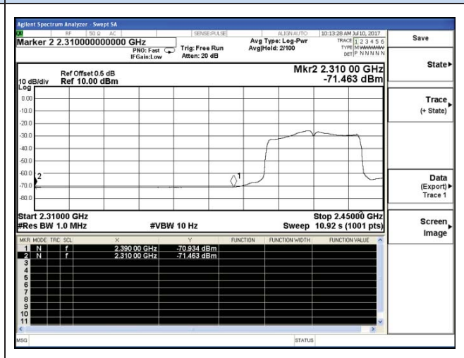
Channel 11 / 2422 MHz – Average IEEE 802.11n HT40
