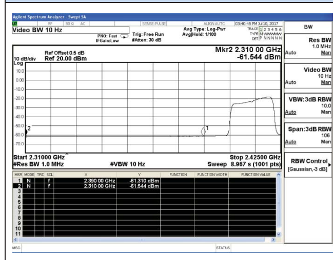
Channel 1 / 2412 MHz – Average IEEE 802.11n HT20
