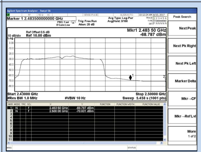
Channel 11 / 2452 MHz – Average
