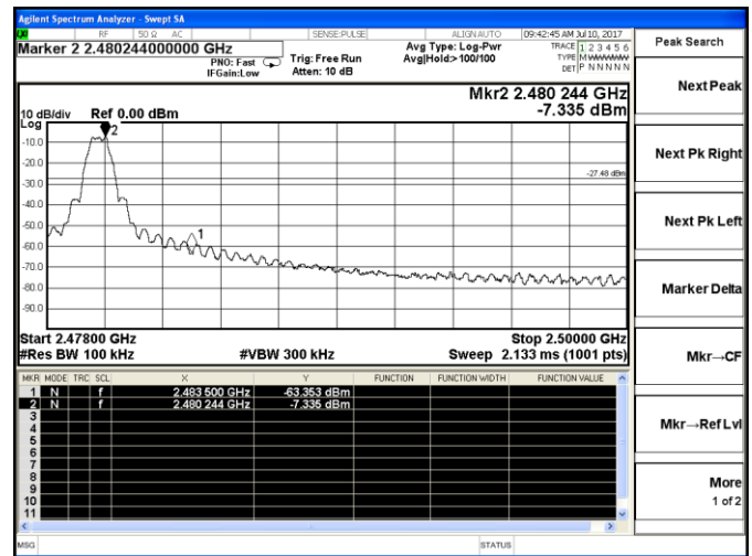
Channel 39 / 2480 MHz
