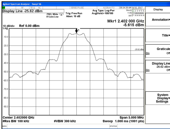
2401 – 2403 MHz
