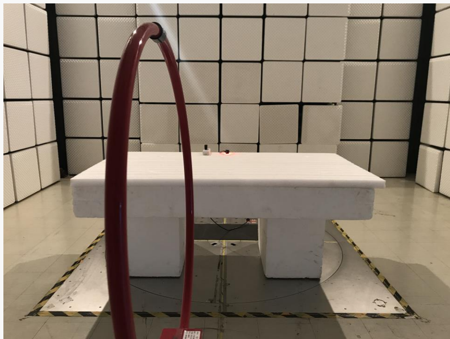
Radiated Emissions - Perpendicular (9kHz – 30MHz)
