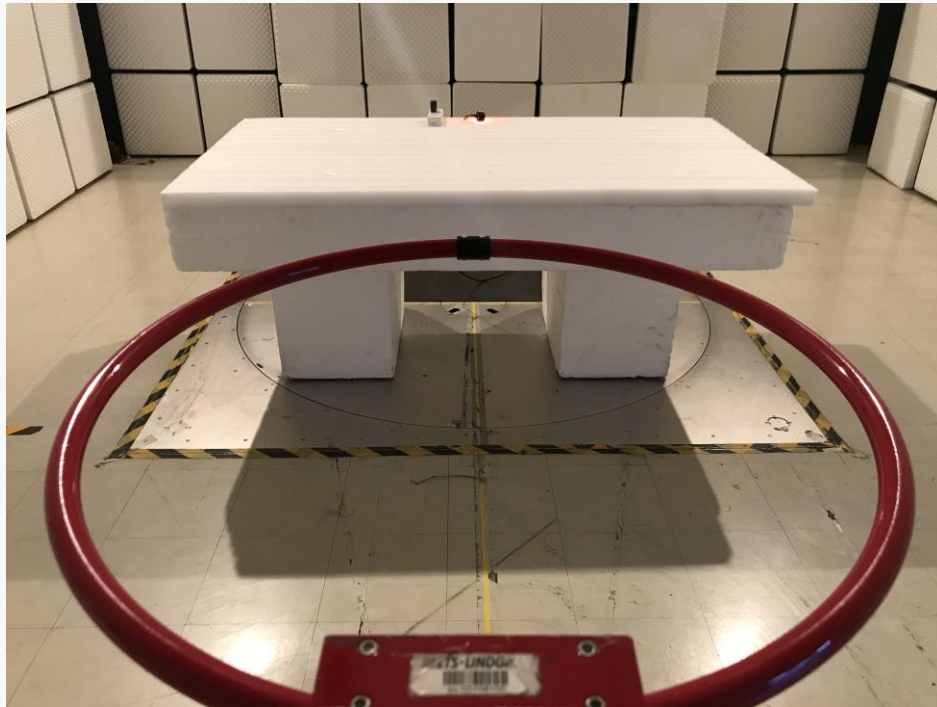
Radiated Emissions - Perpendicular (9kHz – 30MHz)
