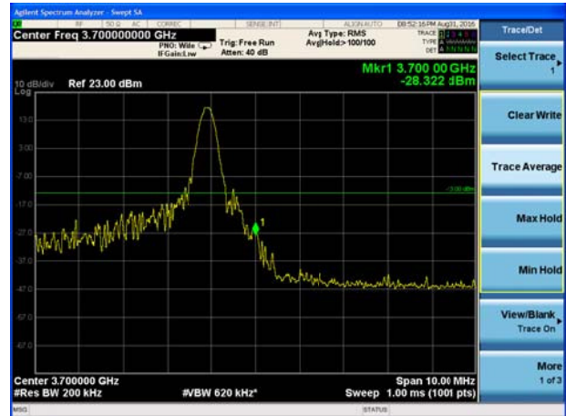
LTE Band 43 16QAM Bandwidth = 20MHz CH44490, RB 1
