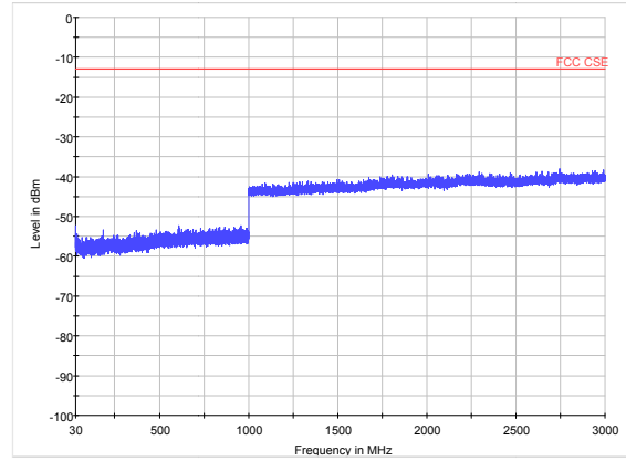
LTE Band 43 10MHz CH44540 30MHz~3GHz
