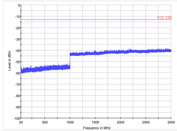
LTE Band 43 20MHz CH44190 30MHz~3GHz
