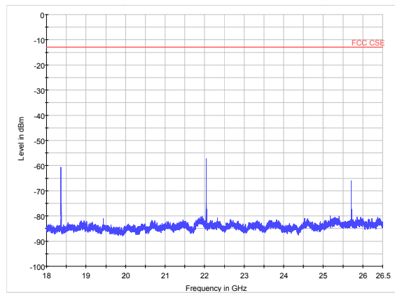
LTE Band 43 5MHz CH44340 18GHz~26.5GHz
