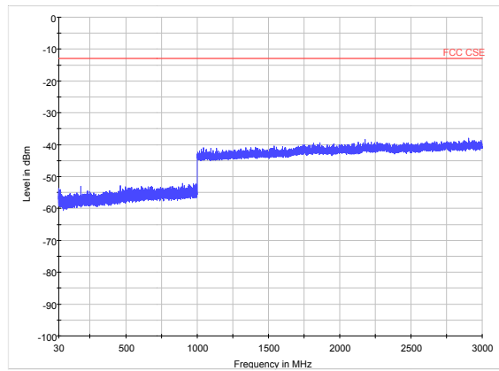
LTE Band 43 5MHz CH44340 30MHz~3GHz
