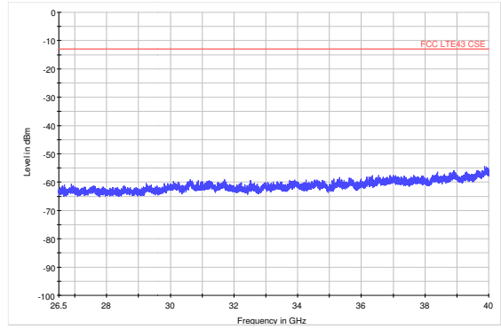
LTE Band 43 20MHz CH44190 26.5GHz~40GHz
