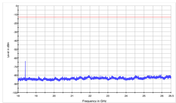
LTE Band 43 20MHz CH44490 18GHz~26.5GHz
