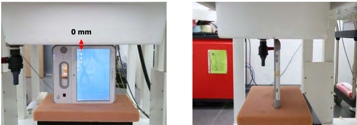
Fig.7 EUT Right side to flat phantom
