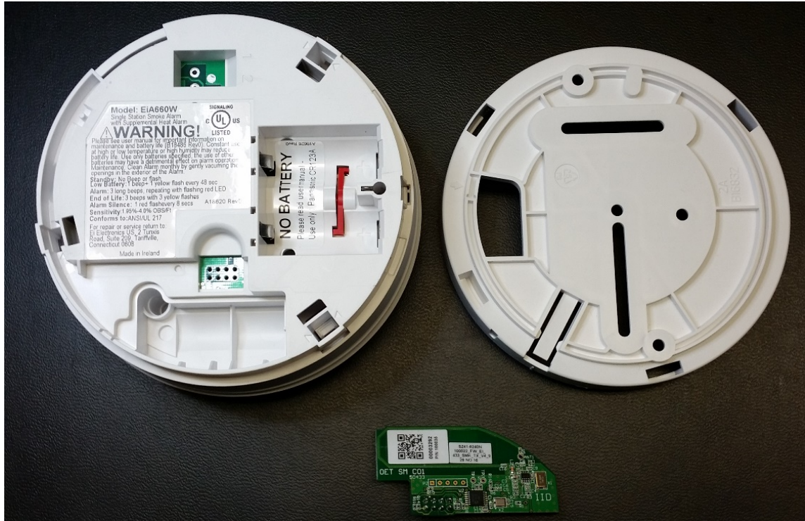
Internal without radio installed
