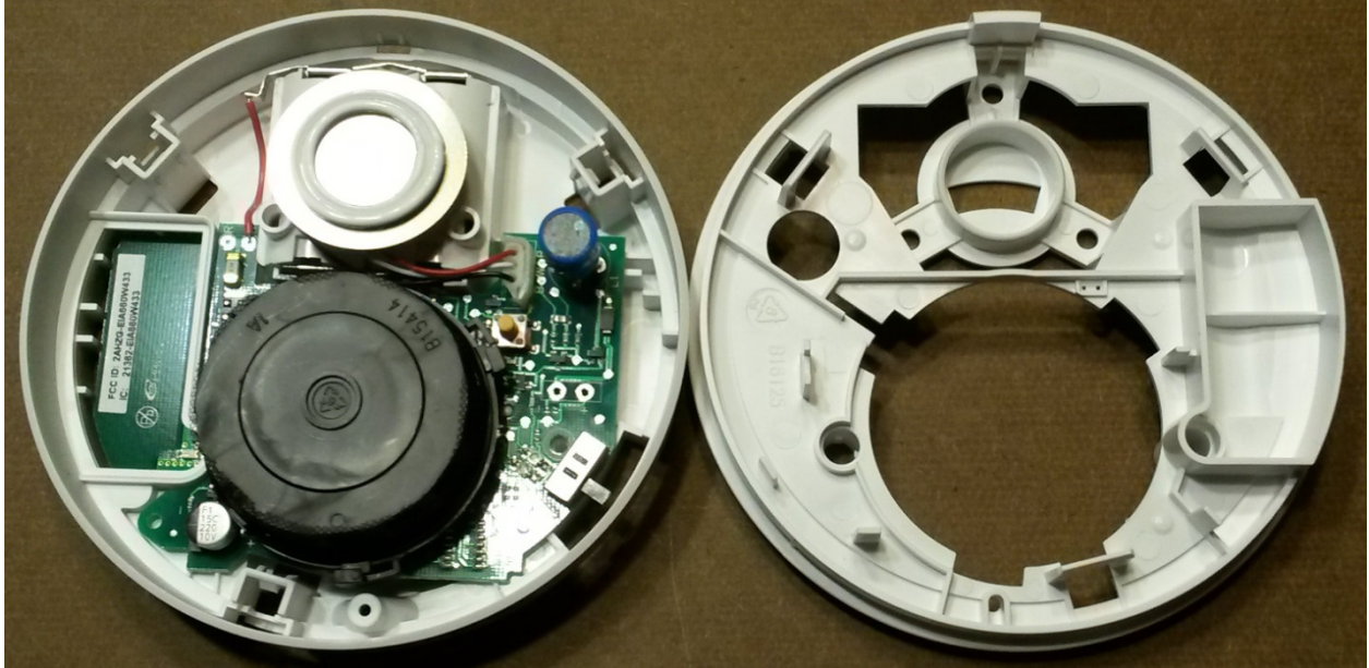
Internal with mid cover removed
