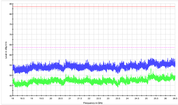
Figure 8.3-13: Spurious emissions within 18–26.5 GHz for SN6250T-F-1-L-G-AC, low channel
