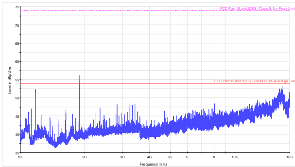
Figure 8.3-11: Spurious emissions within 1–18 GHz for SN6250T-F-1-H-G-DC, high channel
