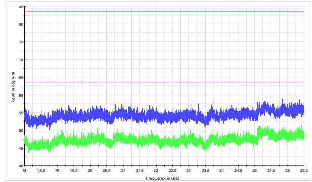
Figure 8.3-14: Spurious emissions within 18–26.5 GHz for SN6250T-F-1-L-G-AC, high channel
