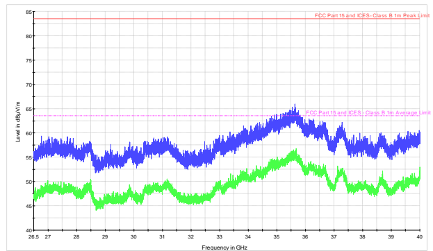
Figure 8.3-18: Spurious emissions within 26.5–40 GHz for SN6250T-F-1-L-G-AC, high channel
