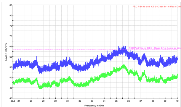
Figure 8.3-17: Spurious emissions within 26.5–40 GHz for SN6250T-F-1-L-G-AC, low channel
