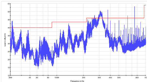
Figure 8.3-5: Spurious emissions below 1 GHz for SN6250T-F-1-H-G-DC, high channel
