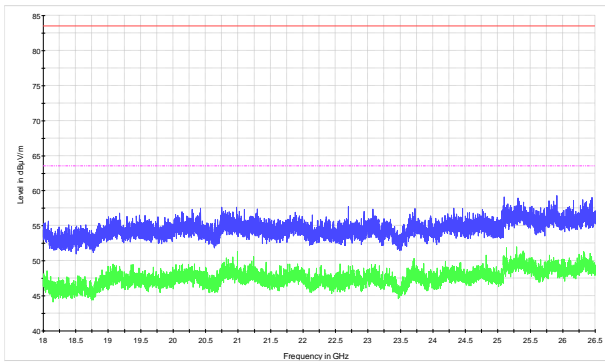
Figure 8.3-15: Spurious emissions within 18–26.5 GHz for SN6250T-F-1-H-G-DC, low channel
