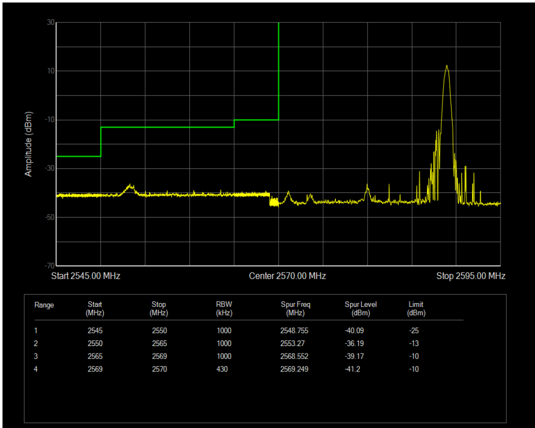
Band41 QAM16 BW=20MHz Channel=40490 RB Size=1 Position=#Max
