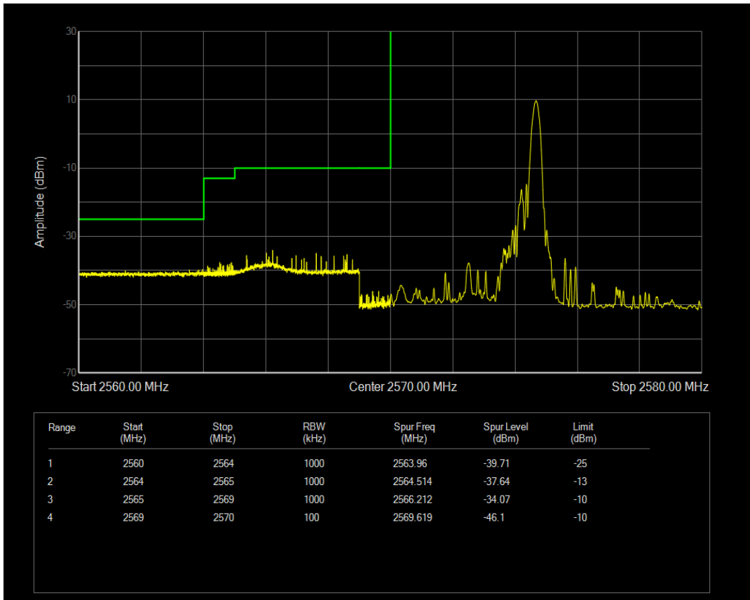
Band41 QAM16 BW=5MHz Channel=40415 RB Size=1 Position=#Max
