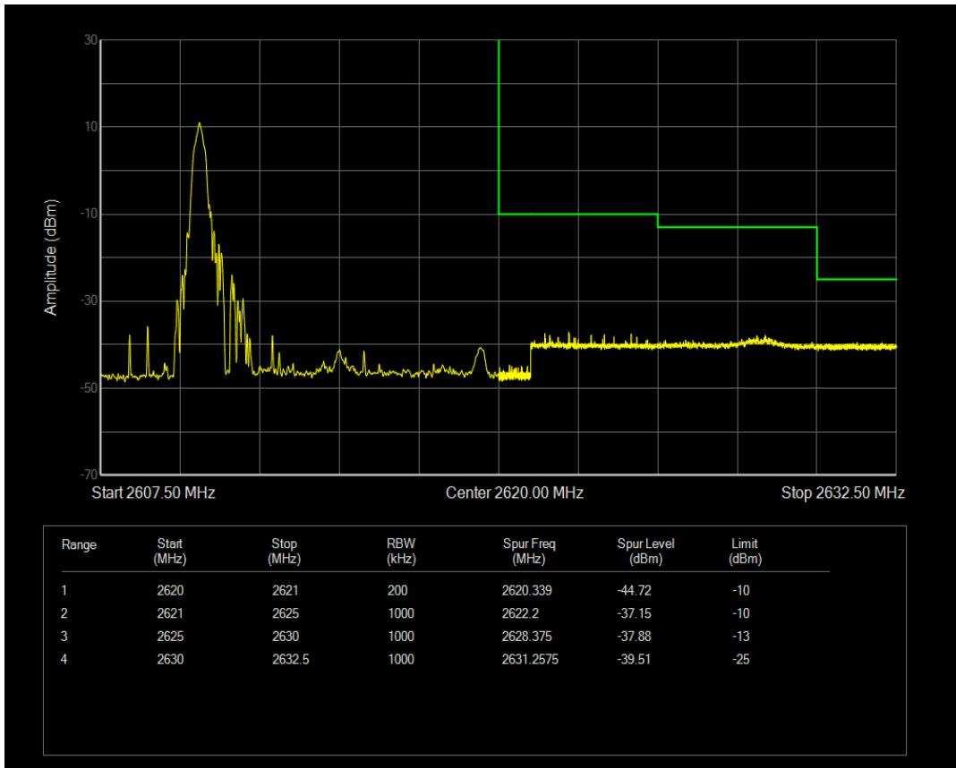
Band41 QAM16 BW=10MHz Channel=40840 RB Size=1 Position=#Max
