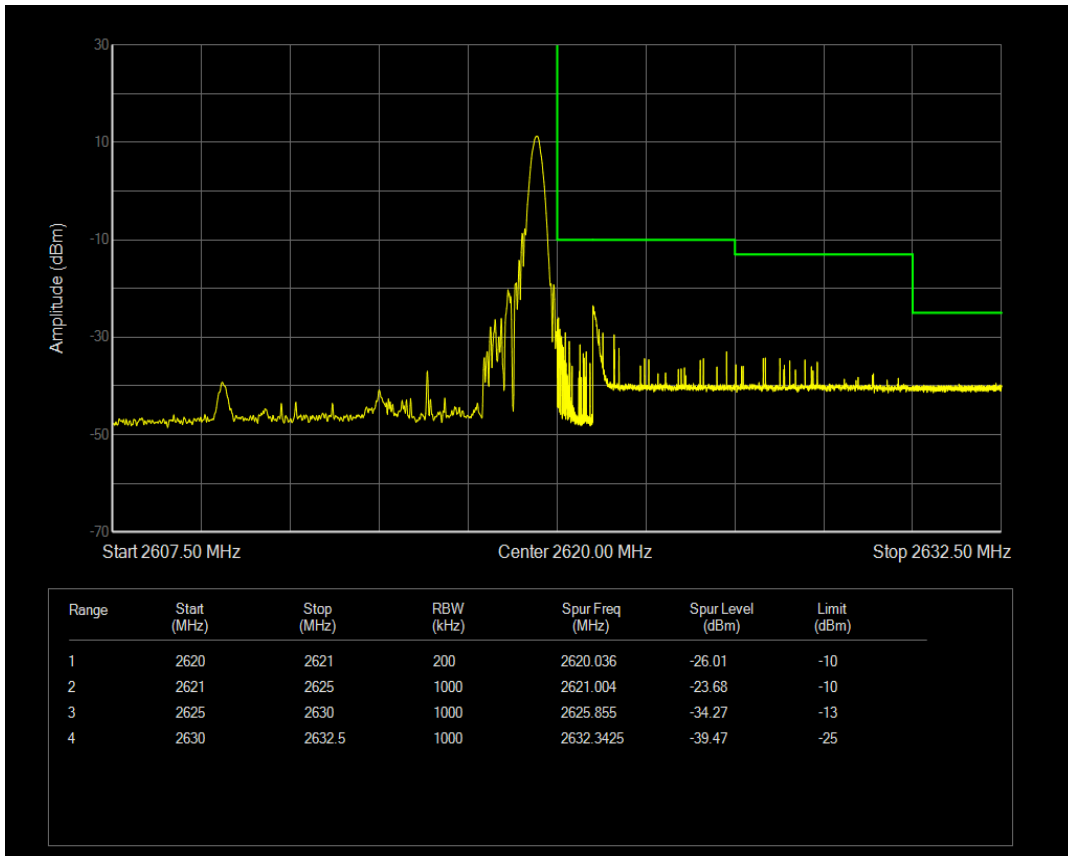
Band41 QAM16 BW=10MHz Channel=40840 RB Size=1 Position=#Max
