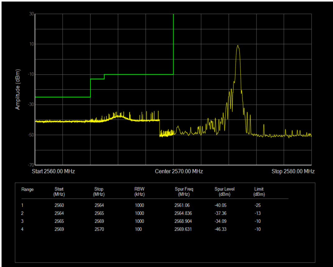
Band41 QAM16 BW=5MHz Channel=40415 RB Size=1 Position=#0
