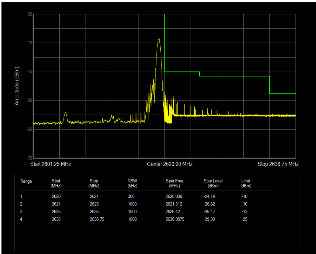
Band41 QPSK BW=15MHz Channel=40815 RB Size=1 Position=#Max
