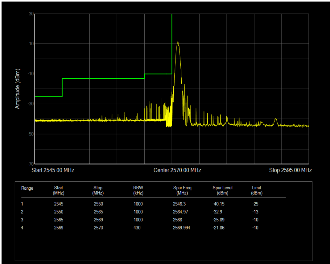
Band41 QAM16 BW=20MHz Channel=40490 RB Size=1 Position=#0
