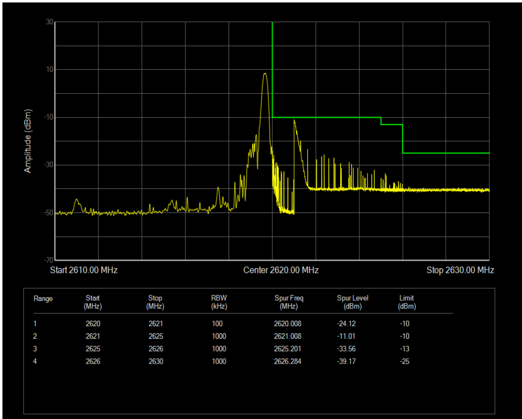
Band41 QAM16 BW=5MHz Channel=40865 RB Size=1 Position=#Max
