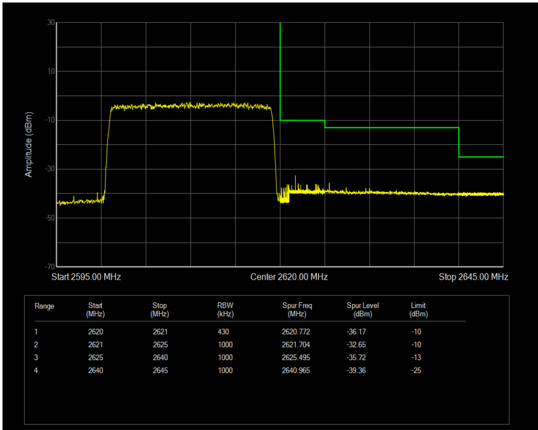
Band41 QPSK BW=20MHz Channel=40790 RB Size=1 Position=#Max
