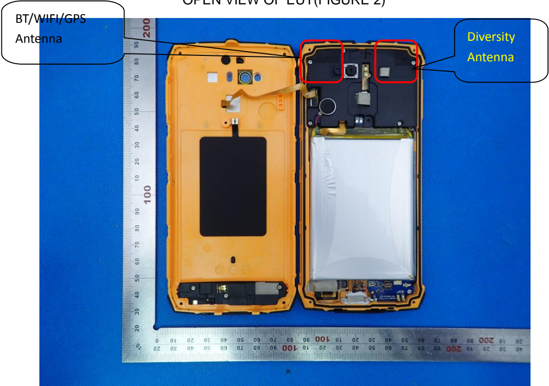
OPEN VIEW OF EUT(FIGURE 2)
