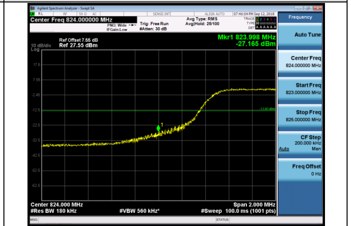
LCH_16QAM_50RB#0
