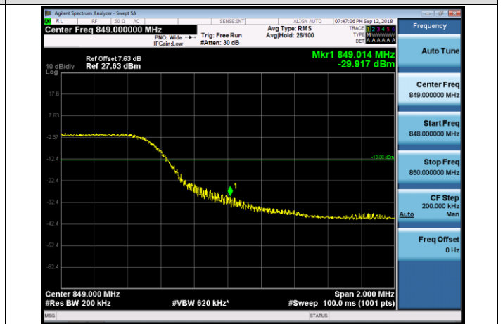
HCH_16QAM_50RB#0
