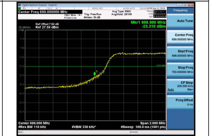
LCH_16QAM_25RB#0
