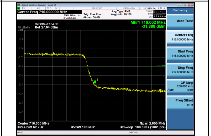
HCH_16QAM_15RB#0
