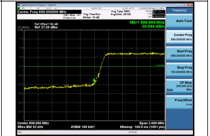
LCH_16QAM_15RB#0
