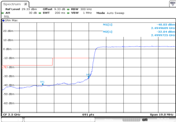
LCH_QPSK_75RB#0
