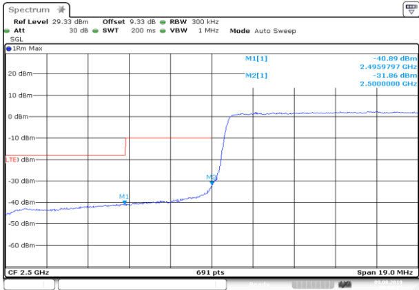
LCH_16QAM_75RB#0
