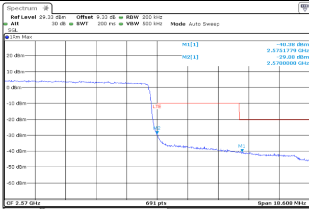
HCH_QPSK_50RB#0
