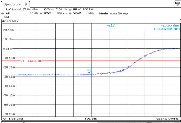
LCH_QPSK_75RB#0
