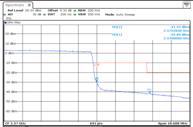
HCH_16QAM_50RB#0
