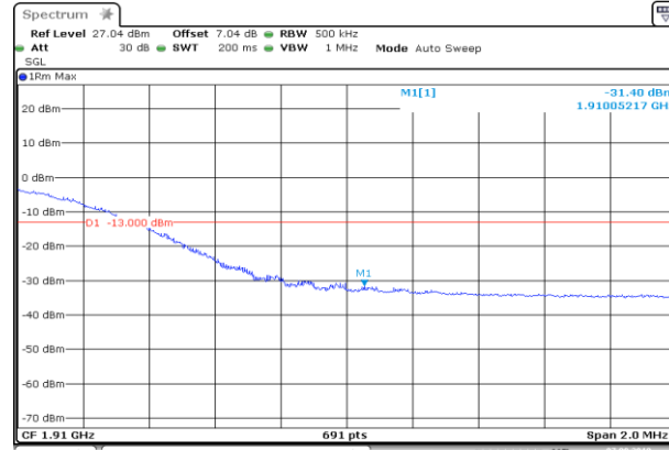
HCH_16QAM_100RB#0
