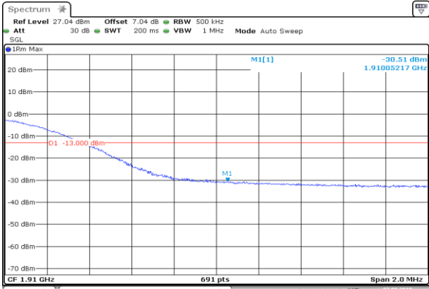
HCH_QPSK_100RB#0
