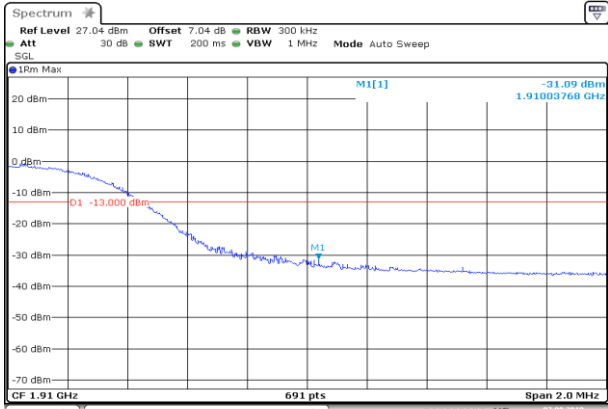
HCH_16QAM_75RB#0
