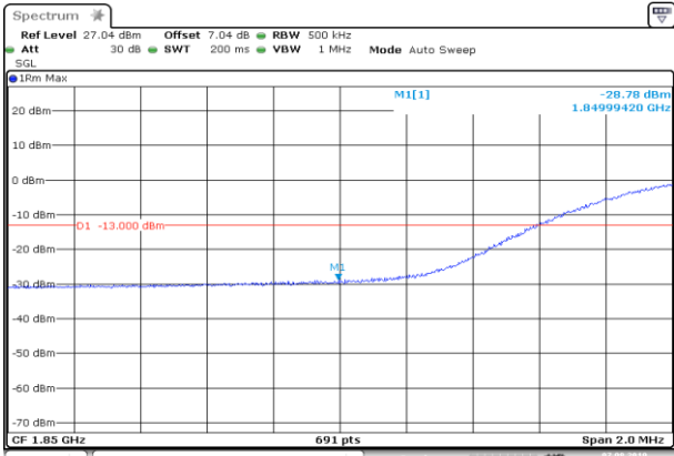
LCH_QPSK_100RB#0
