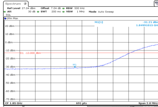
LCH_16QAM_100RB#0
