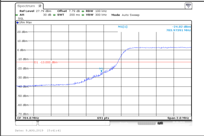
LCH_QPSK_25RB#0
