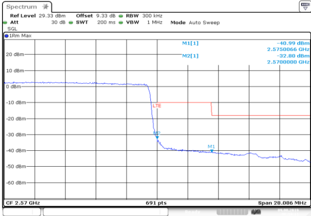
HCH_16QAM_75RB#0
