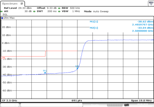
LCH_QPSK_100RB#0
