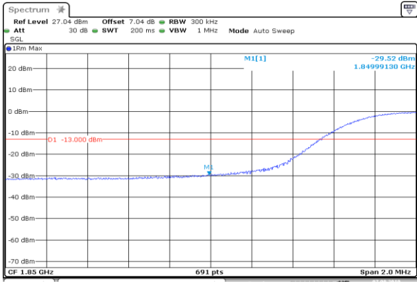
LCH_16QAM_75RB#0
