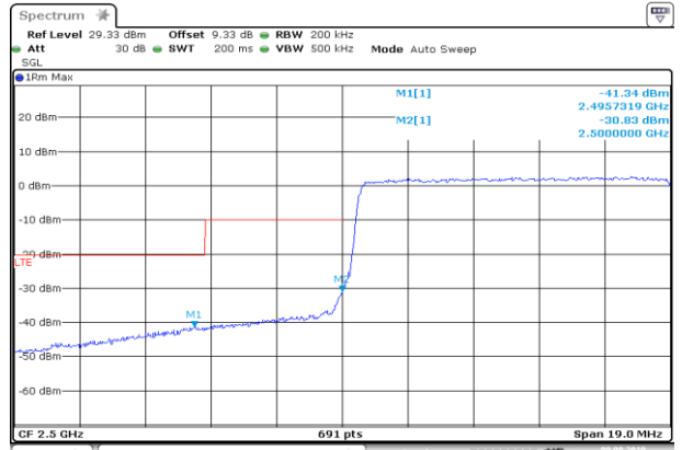
LCH_16QAM_50RB#0
