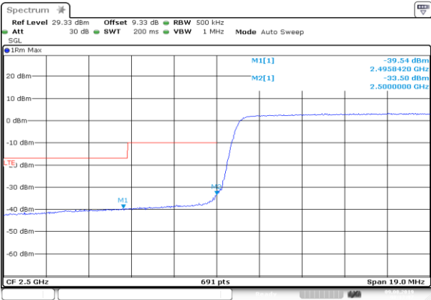
LCH_16QAM_100RB#0
