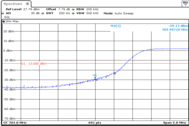
LCH_16QAM_50RB#0
