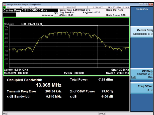
5814MHz-ANT B
