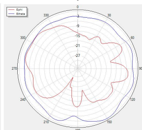
Phi=90 freq=2440MHz
