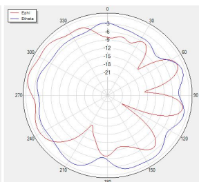
Phi=90 freq=2480MHz
