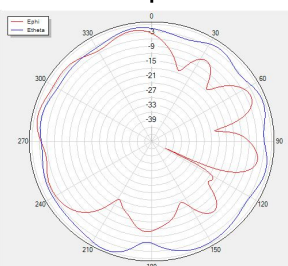
Phi=90 freq=2480MHz
