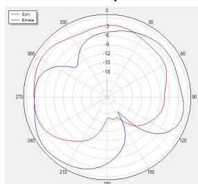
Theta=90 freq=2480MHz
