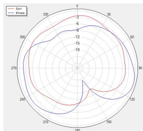
Theta=90 freq=2440MHz
