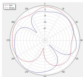
Theta=90 freq=2480MHz
