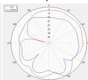
Phi=0 freq=2440MHz
