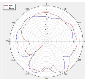
Phi=0 freq=2480MHz
