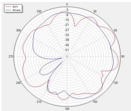
Phi=90 freq=2400MHz
