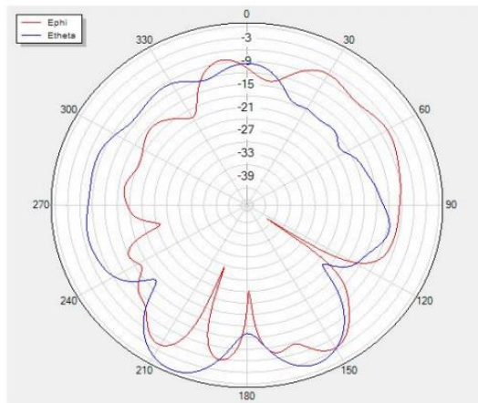
Phi=0 freq=2400MHz
