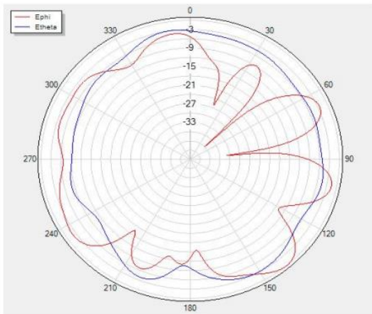
Phi=90 freq=2400MHz
