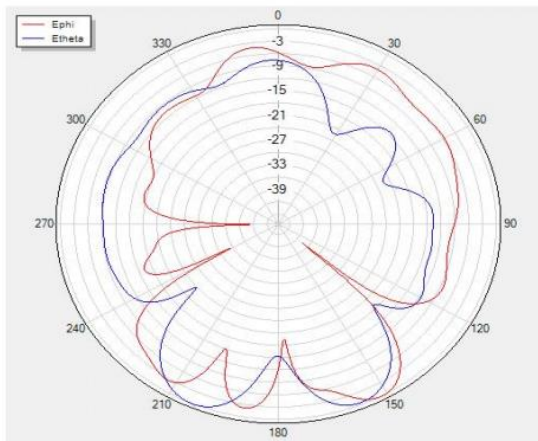
Phi=0 freq=2400MHz
