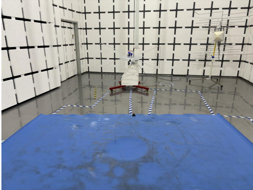
Radiated Emissions (30MHz-1GHz) R-ear
