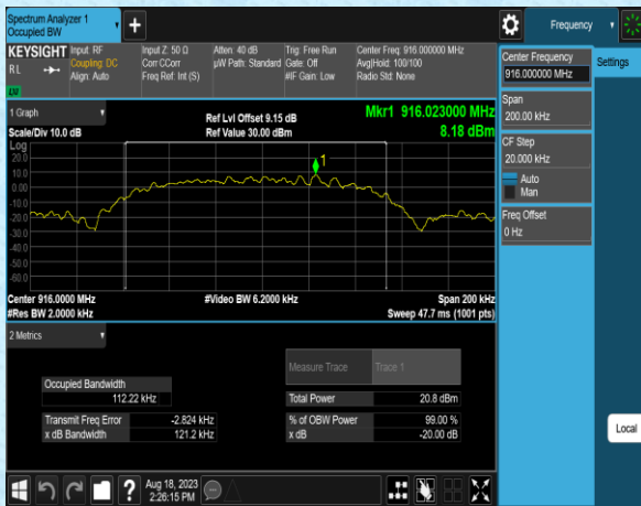
916MHz
