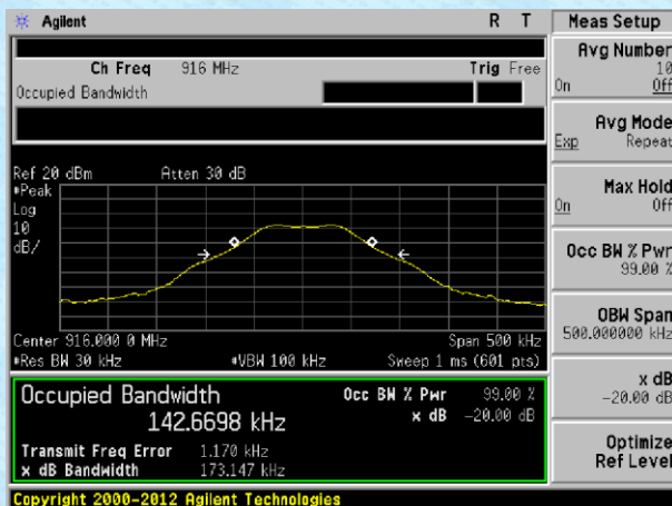
916MHz
