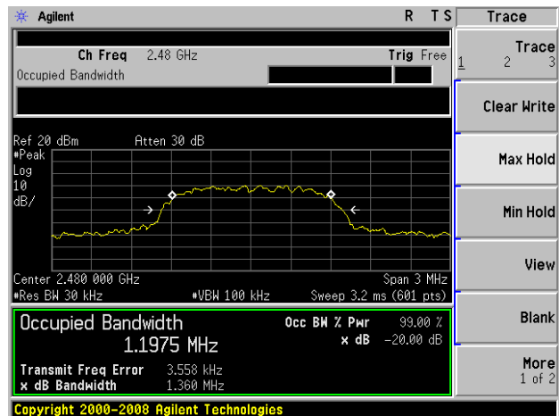
20dB Bandwidth plot on channel 78 (2Mbps)
