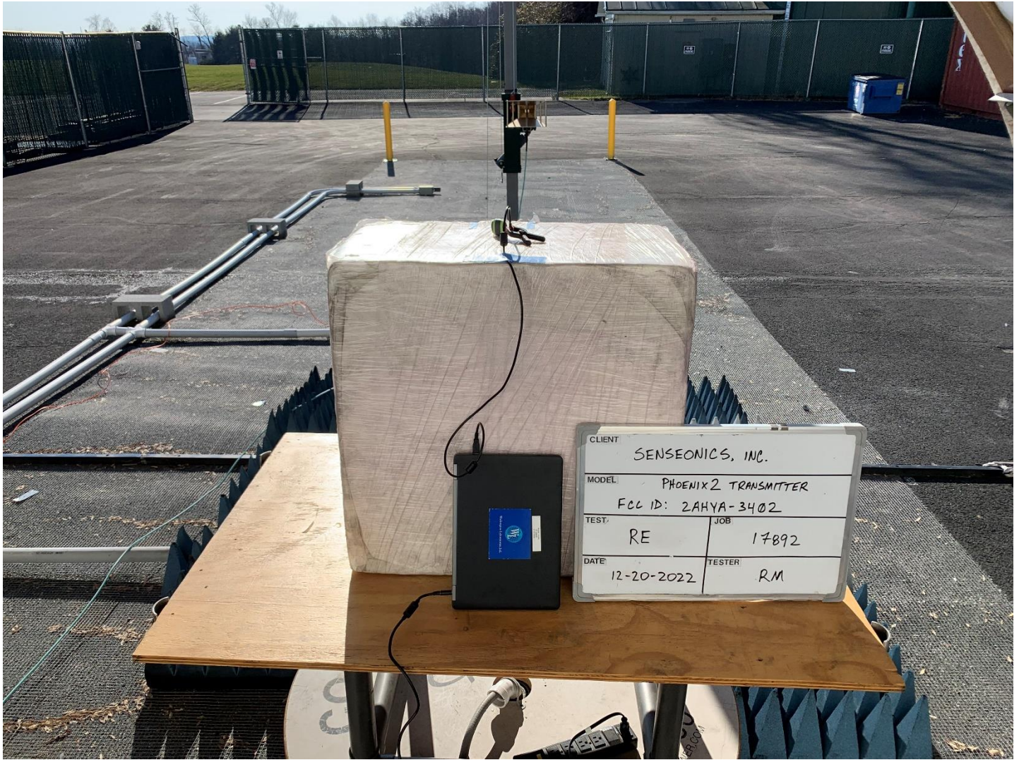
Radiated Emissions Rear View, > 1GHz
