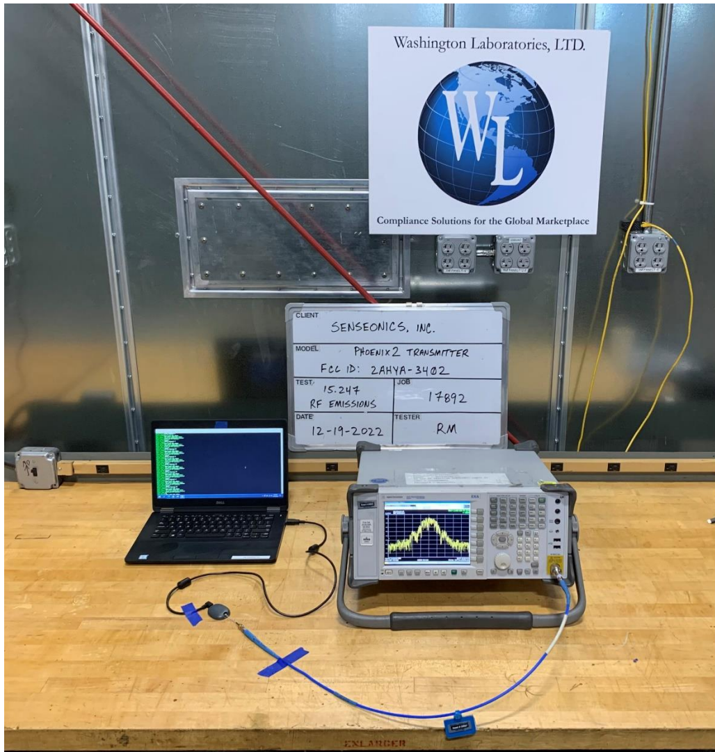
Benchtop Conducted RF Emissions
