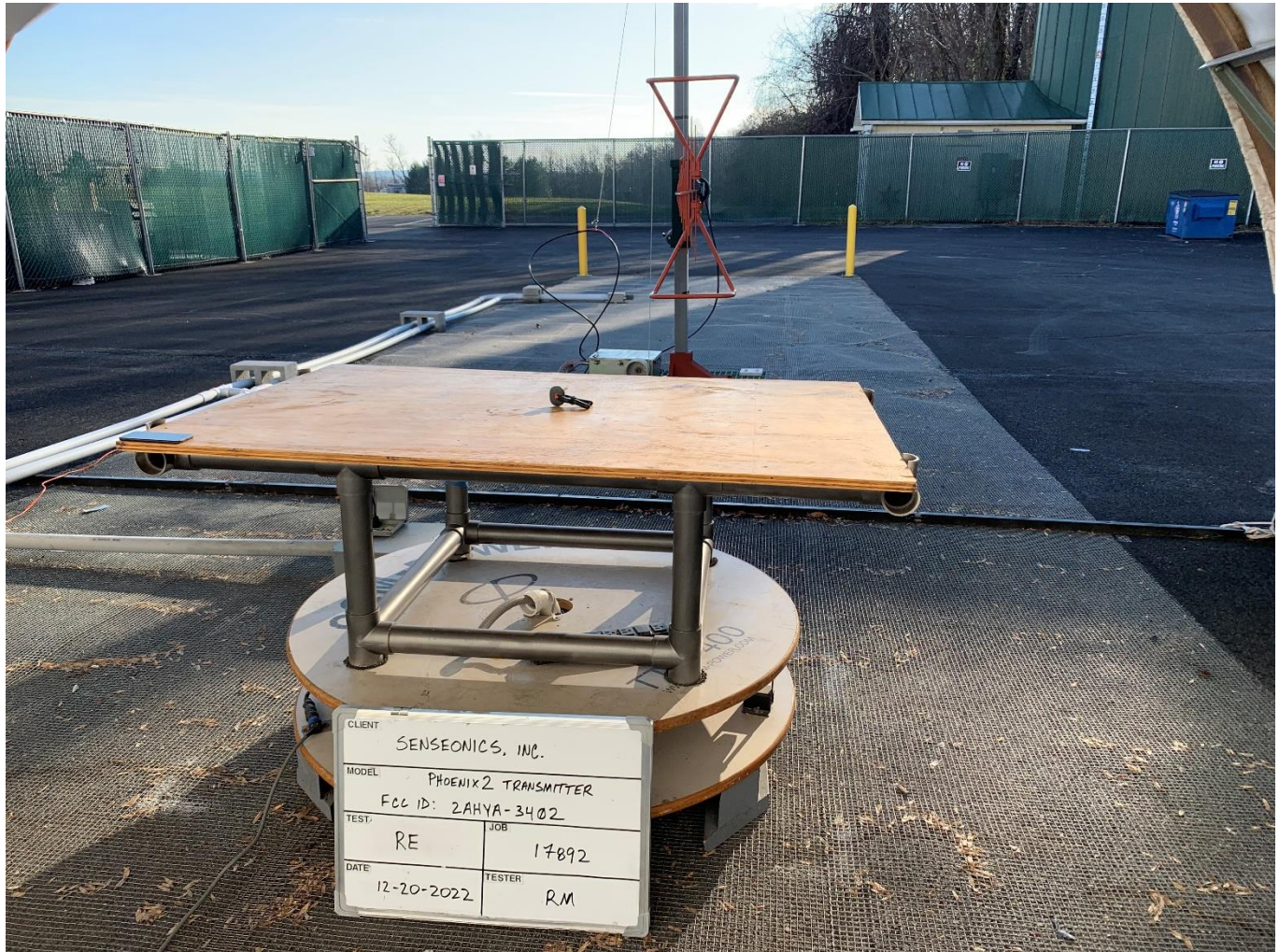
Radiated Emissions Rear View, < 1GHz
