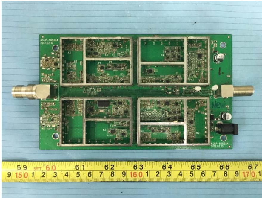
EUT – Main Board Top Shilded off View
