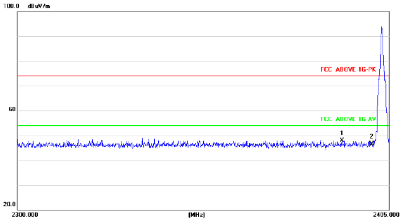
2402MHz Vertical
