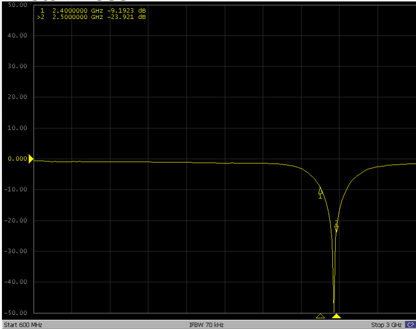
Return loss
